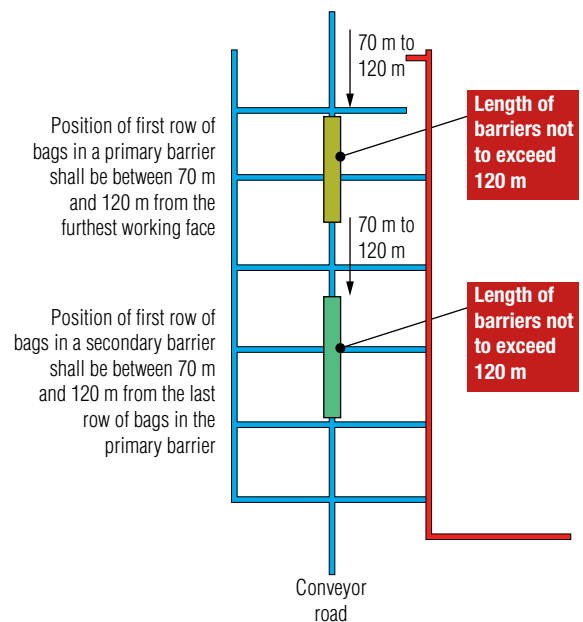
Figure 4b Protection of an established bord and pillar working using primary and secondary barriers
